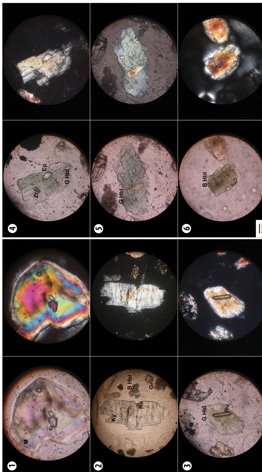
Plate. Heavy minerals identified in the studied samples; left images in plain light; right images in crossed-polarized light; M – muscovite; Ky – kyanite; Ru – rutile; Gr – garnet; B, G Hbl – brown, green hornblende; Zr – zircon.
