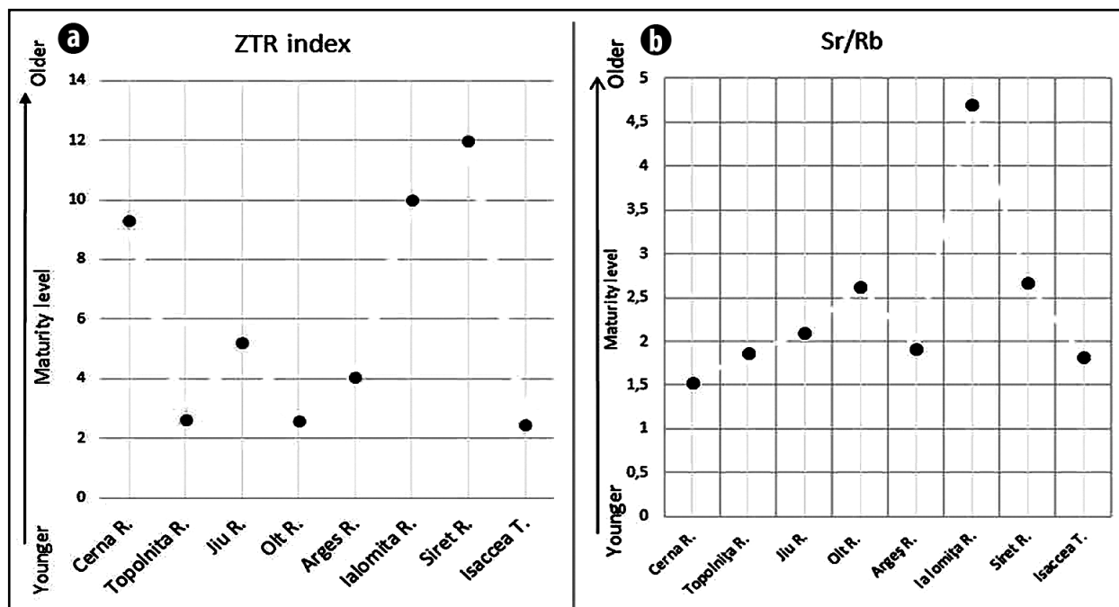
Fig. 6. Diagrams showing relative maturity of the studied samples (this study): (a) ZTR (zircon + tourmaline + rutile) index; (b) Sr/Rb ratio.
