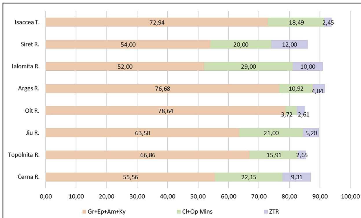
Fig. 5. HM association concentration and ZTR index (zircon + tourmaline + rutile) values in the sampled river confluence with the Danube
