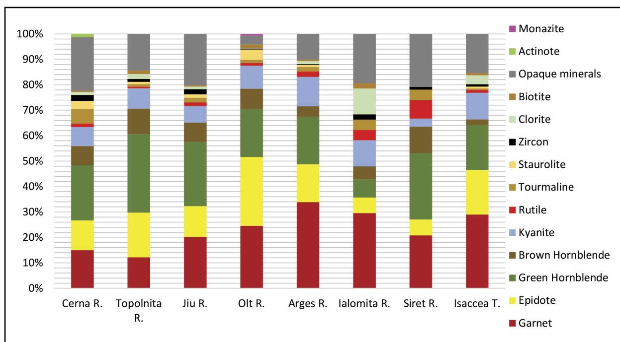
Fig. 4. Heavy mineral abundances of the sampled locations.
