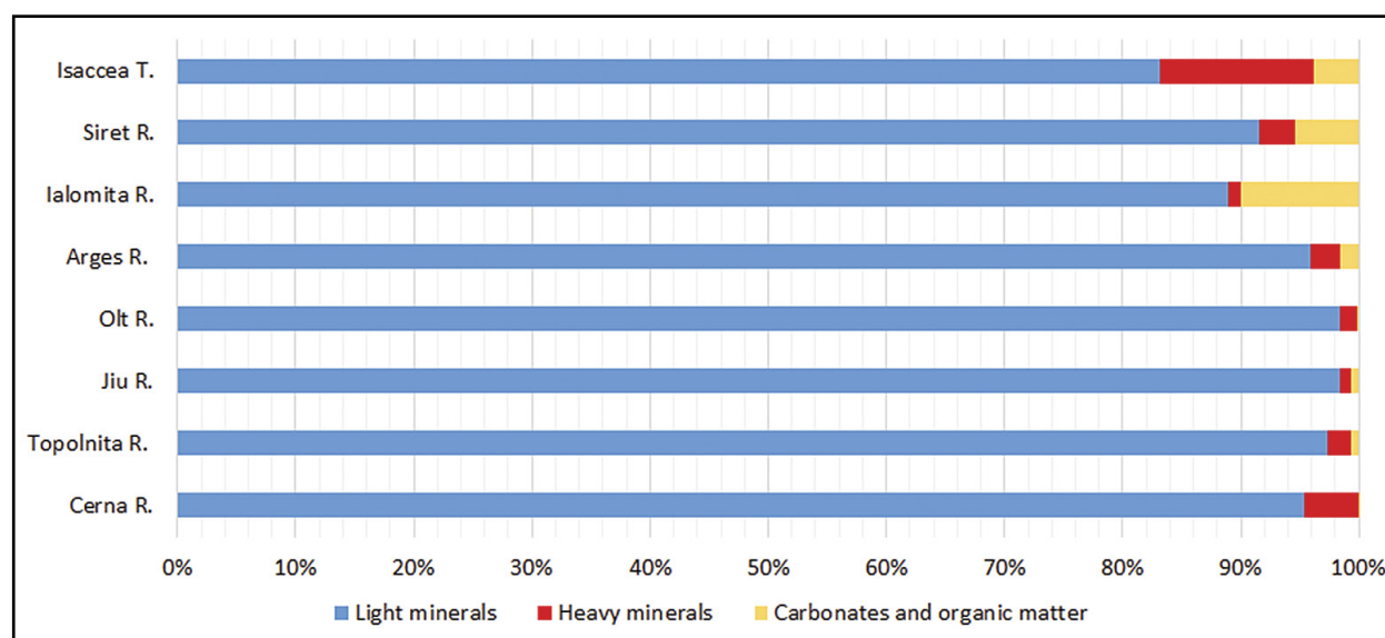
Fig. 3. Concentration of the light and heavy minerals and of the carbonates and organic matter.
