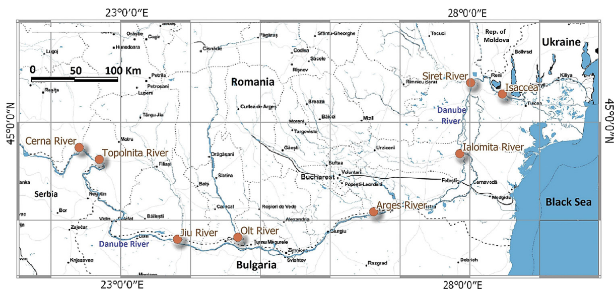
Fig. 1. The Lower Danube course and the location of the studied samples (from https://www.openstreetmap.org )
