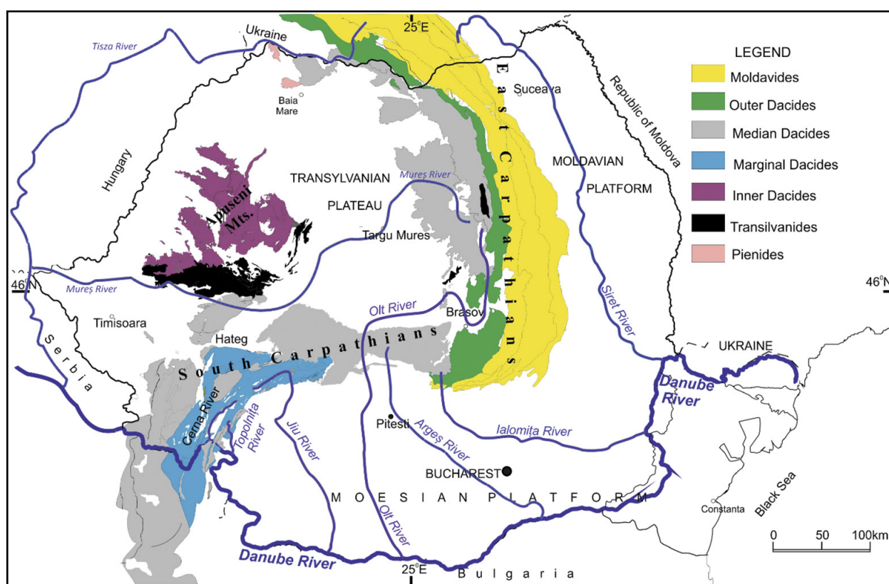
Fig. 2. Tectonic map of Romania (from Melinte-Dobrinescu et al. , 2009 modified after Săndulescu, 1984; Bădescu, 2005) and the sampled Danube River left tributaries.
